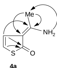
Fig. 1 HMBC correlations used in the structure elucidation of 4a (the correlation between the NH 2 protons and the methyl C atom was established by selective decoupling)
